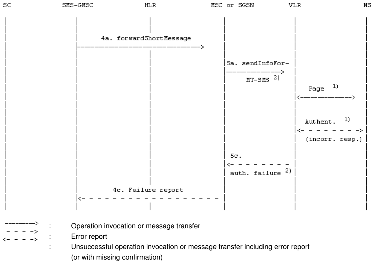
Figure 16c): "Send information for MT SMS" procedure; erroneous case: Absent subscriber (e.g. no paging response)
