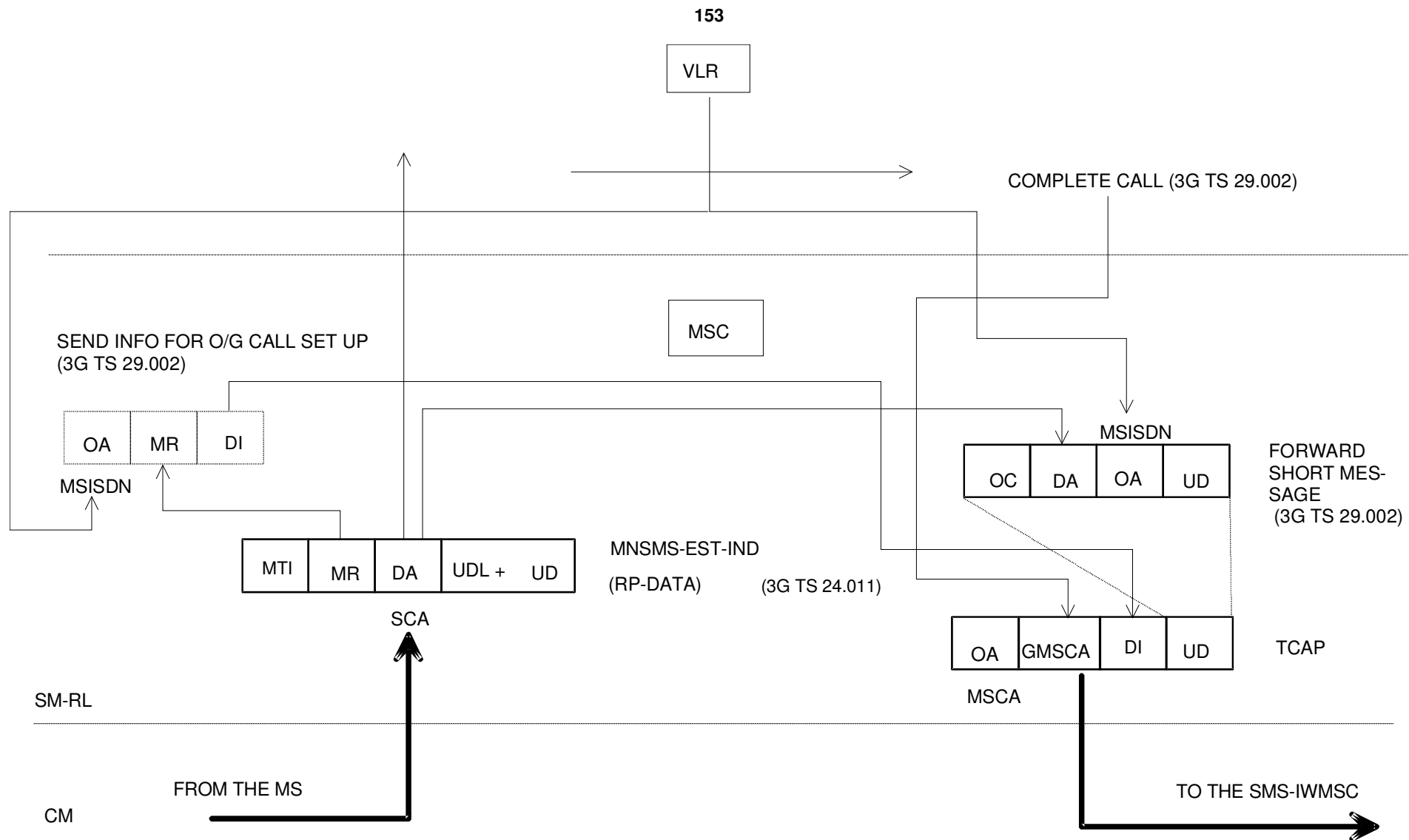
Figure C.10: Mobile originated short message
