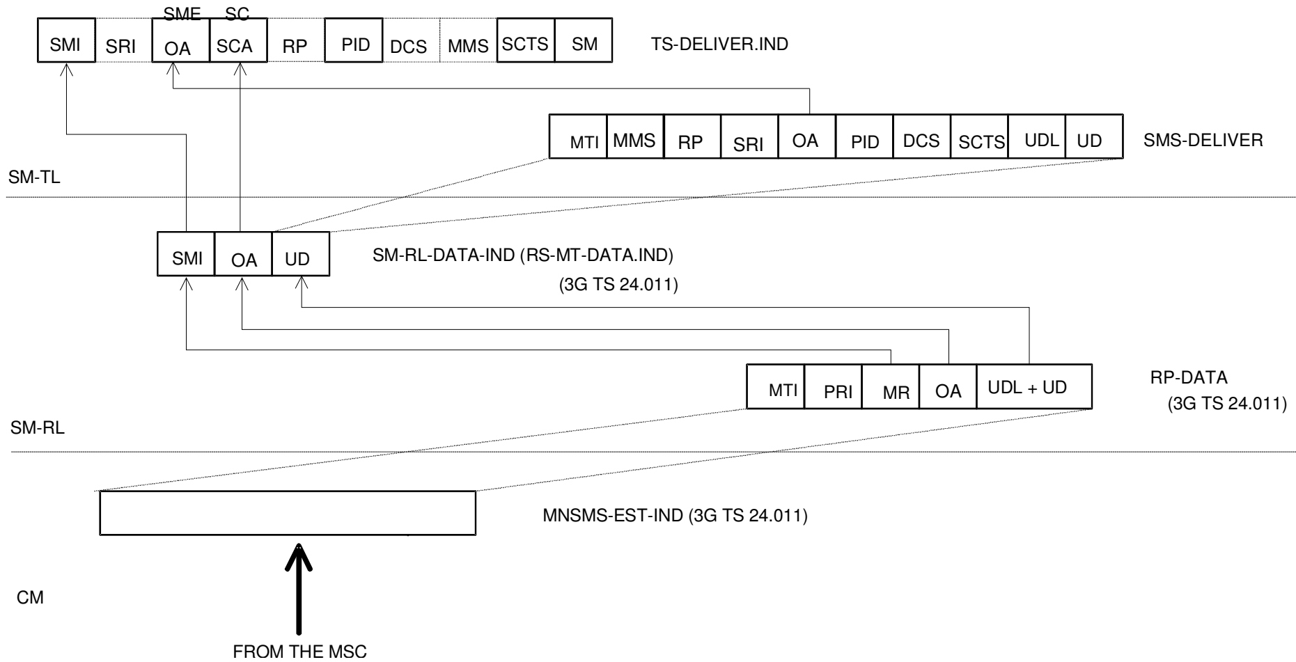
Figure C.4: Mobile terminated short message
