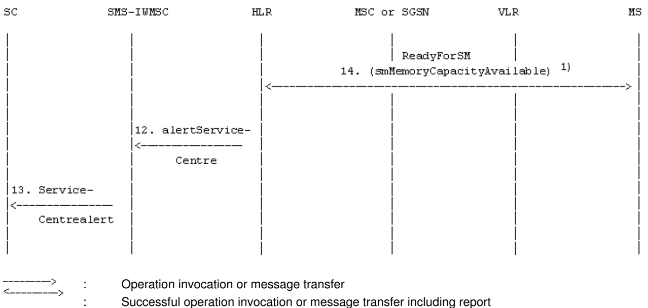
Figure 20b: The alert procedure when the MS becomes reachable, MNRF, MNRG or both are set and MCEF is set
