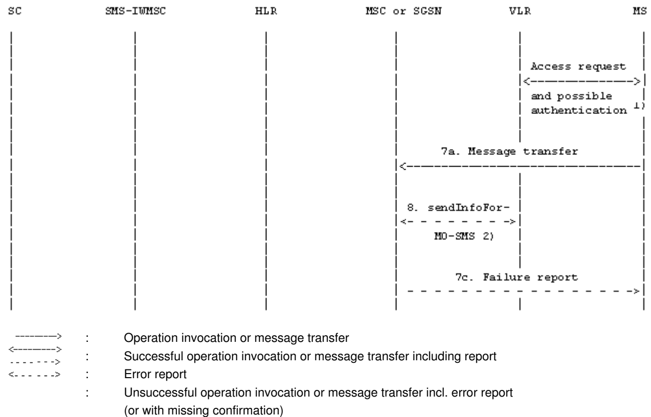
Figure 18b): Short message transfer attempt failing due to error at the MSC or SGSN
